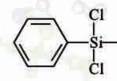
Methylphenyldichlorosilane
